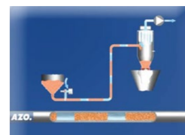
Dense Phase
