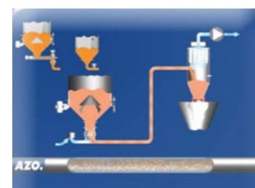
Dilute Phase
