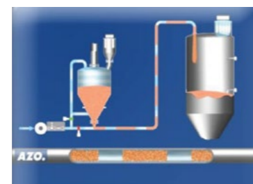
Dense Phase
